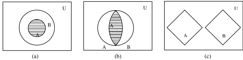
Fig. 4: Venn diagram for intersection of sets
