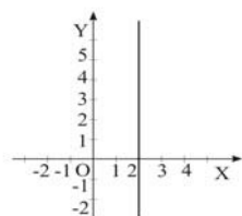
Fig. 8(a): \{2\} \times \mathbf{R} , i.e., x=2
