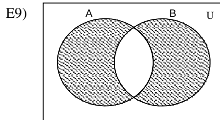
Fig. 12: The Shaded portion is A \Delta B
