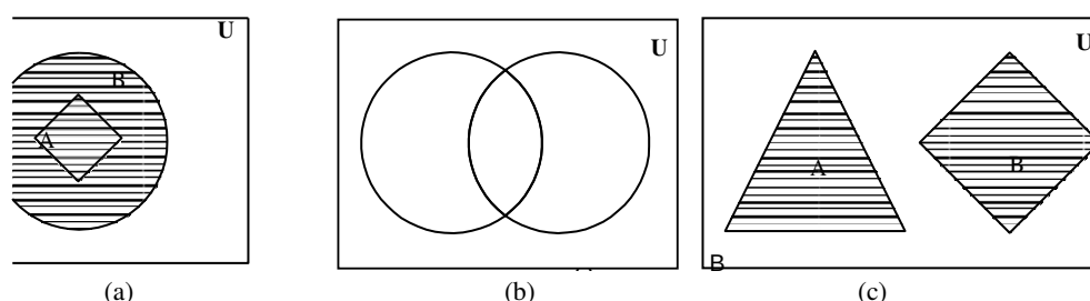
Fig.3: Venn diagram for union
